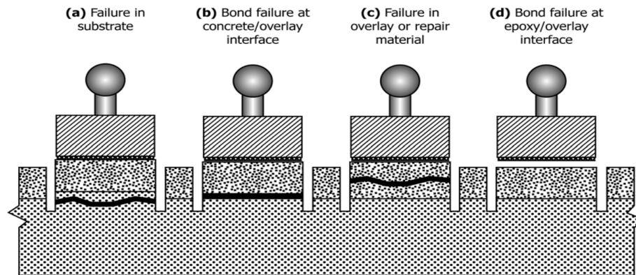
FIG. 3 Schematic of Failure Modes
